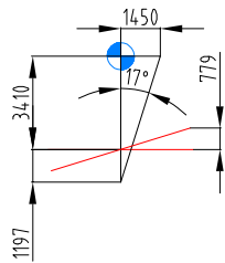
Geometric Trimming Diagram 稳定角
